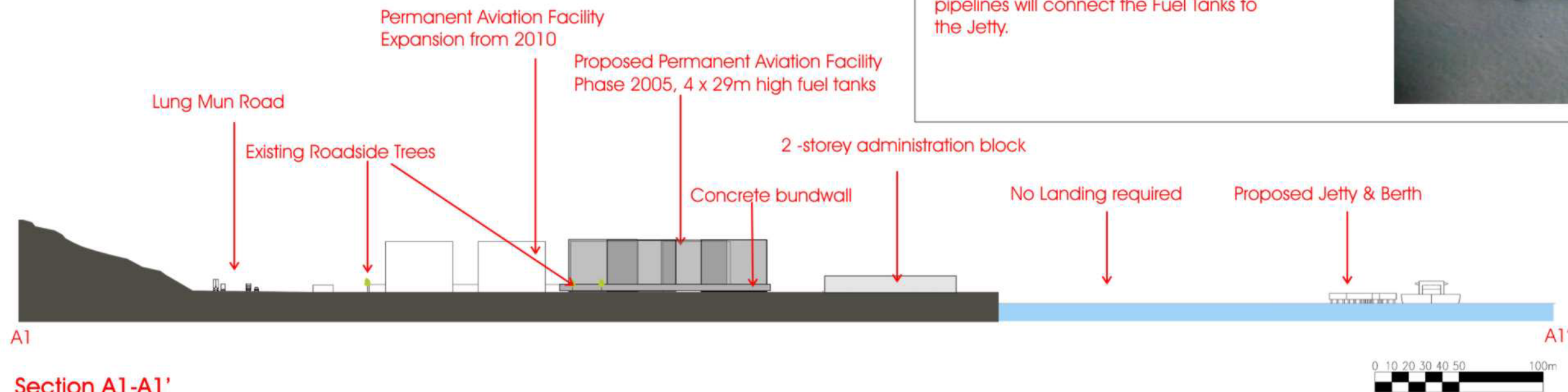
Indicative Section of the Proposed Permanent Aviation Facility and Jetty
