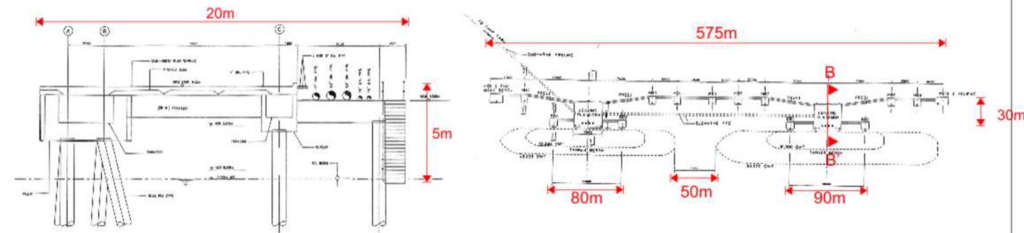
Plan & Elevation of Proposed PAFF Jetty
